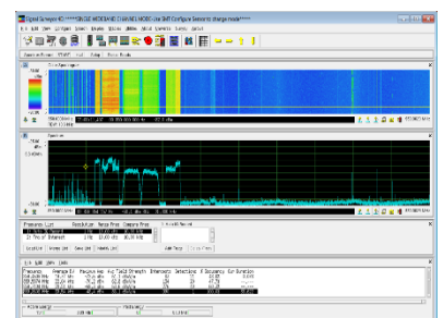
Portable monitoring system covering VLF to 5G millimeter wave bands
